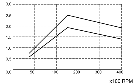
KW Power KW / Speed (R.P.M)
