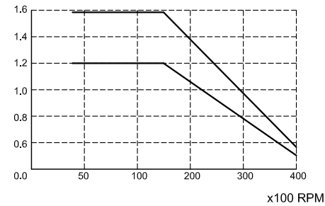
Nm Torque Nm / Speed (R.P.M)
